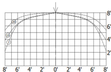
1/2" Orifice - K=5.6
